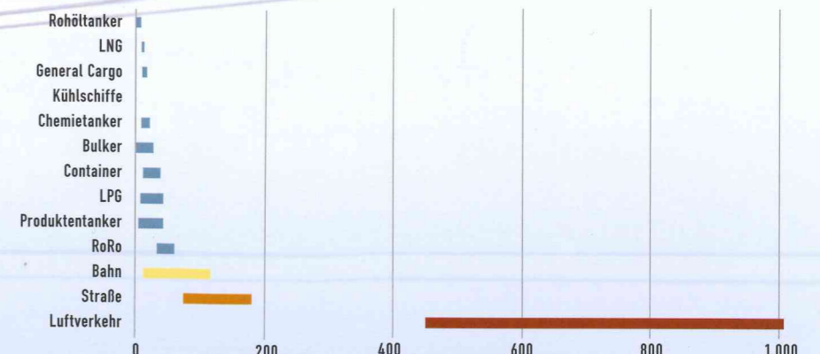
Quelle: Second IMO GHG Study 2009
